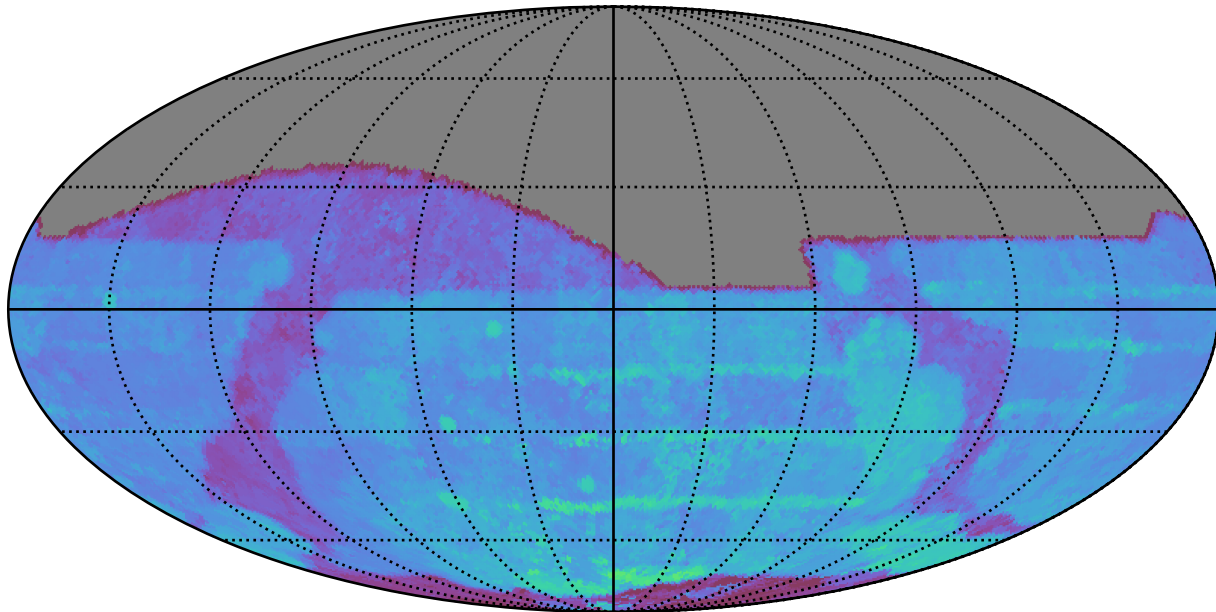
too_100_1v3.4_10yrs All sky r band: 80thPercentile Season Length
