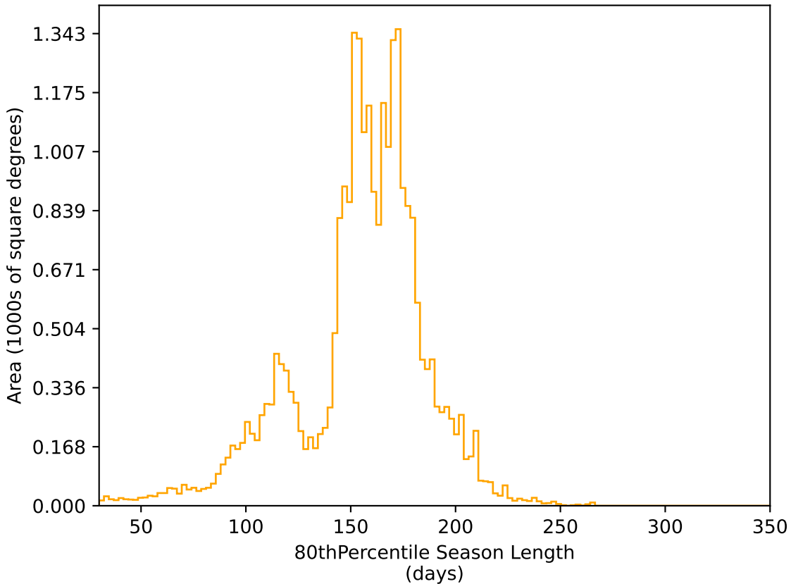
too_100_1v3.4_10yrs All sky r band: 80thPercentile Season Length
