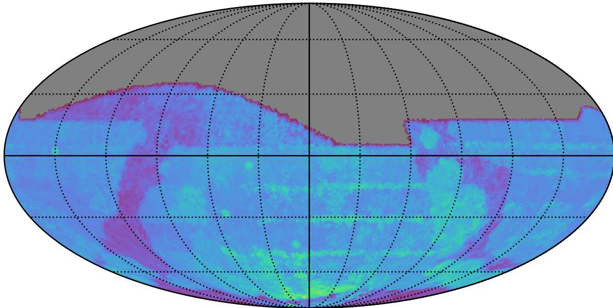
too_100_1v3.4_10yrs All sky i band: 80thPercentile Season Length
