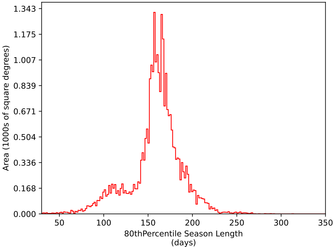
too_100_1v3.4_10yrs All sky i band: 80thPercentile Season Length
