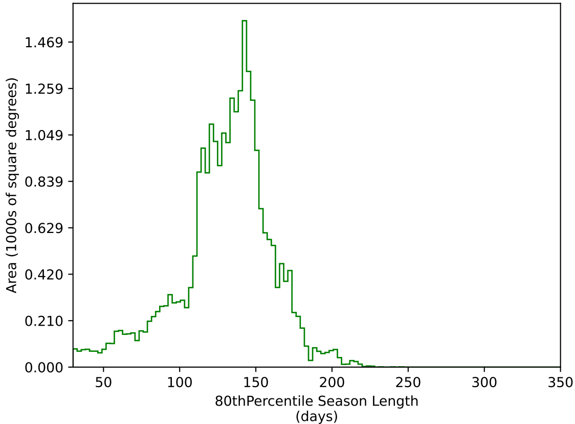
too_100_1v3.4_10yrs All sky g band: 80thPercentile Season Length
