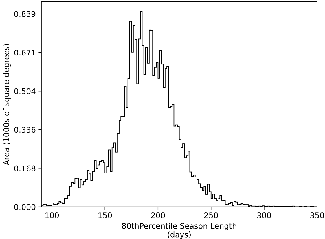
too_100_1v3.4_10yrs All sky all bands: 80thPercentile Season Length
