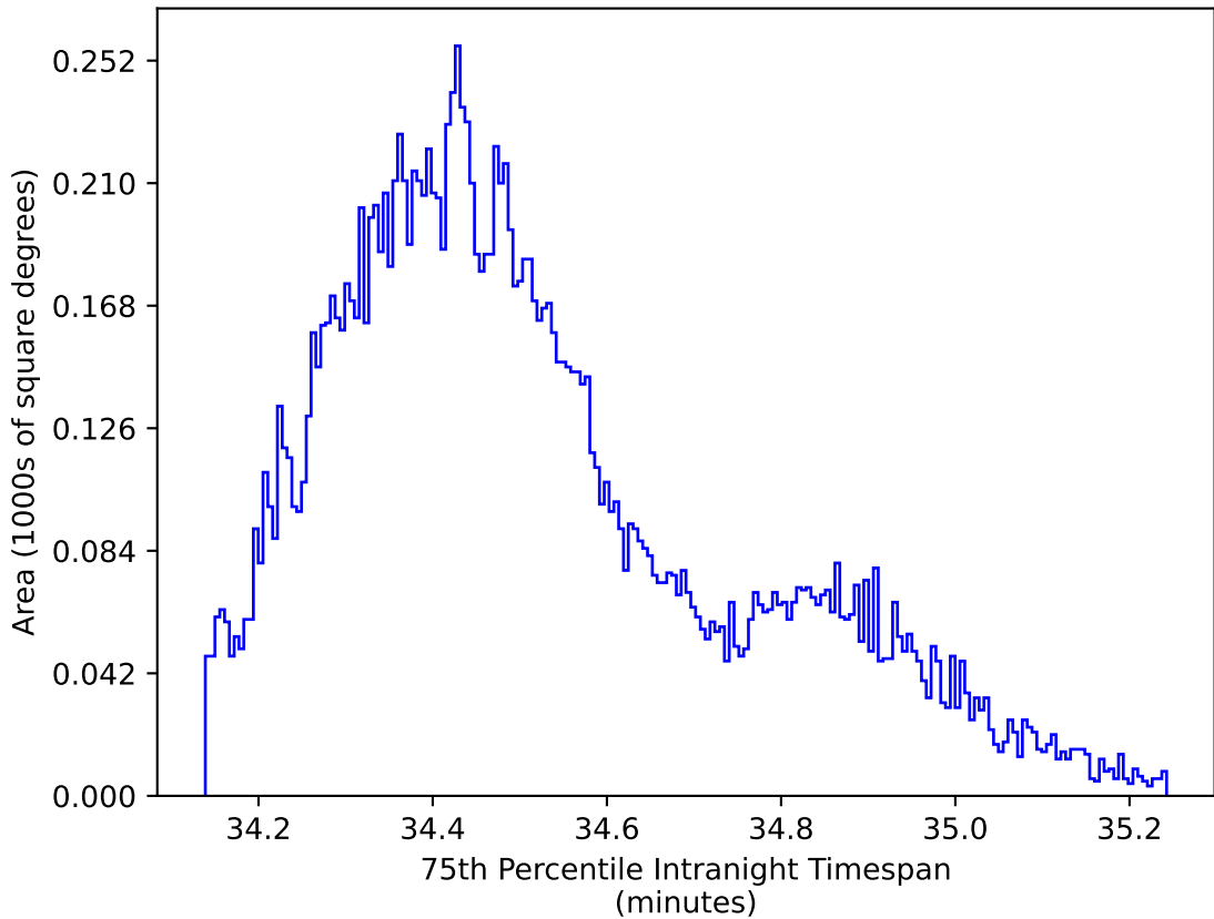
too_100_1v3.4_10yrs WFD zy bands: 75th Percentile Intranight Timespan
