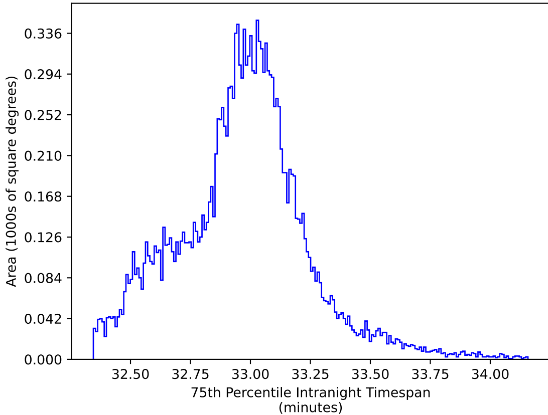
too_100_1v3.4_10yrs WFD y band: 75th Percentile Intranight Timespan
