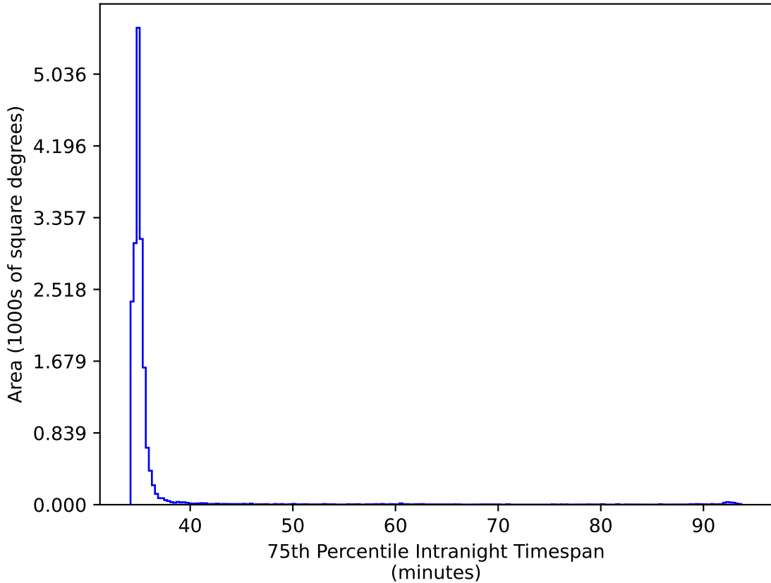
too_100_1v3.4_10yrs WFD ri bands: 75th Percentile Intranight Timespan
