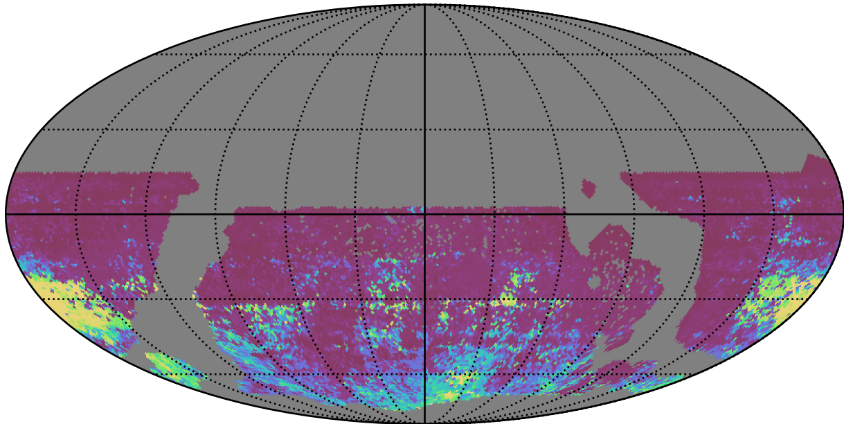
too_100_1v3.4_10yrs WFD r band: 75th Percentile Intranight Timespan
