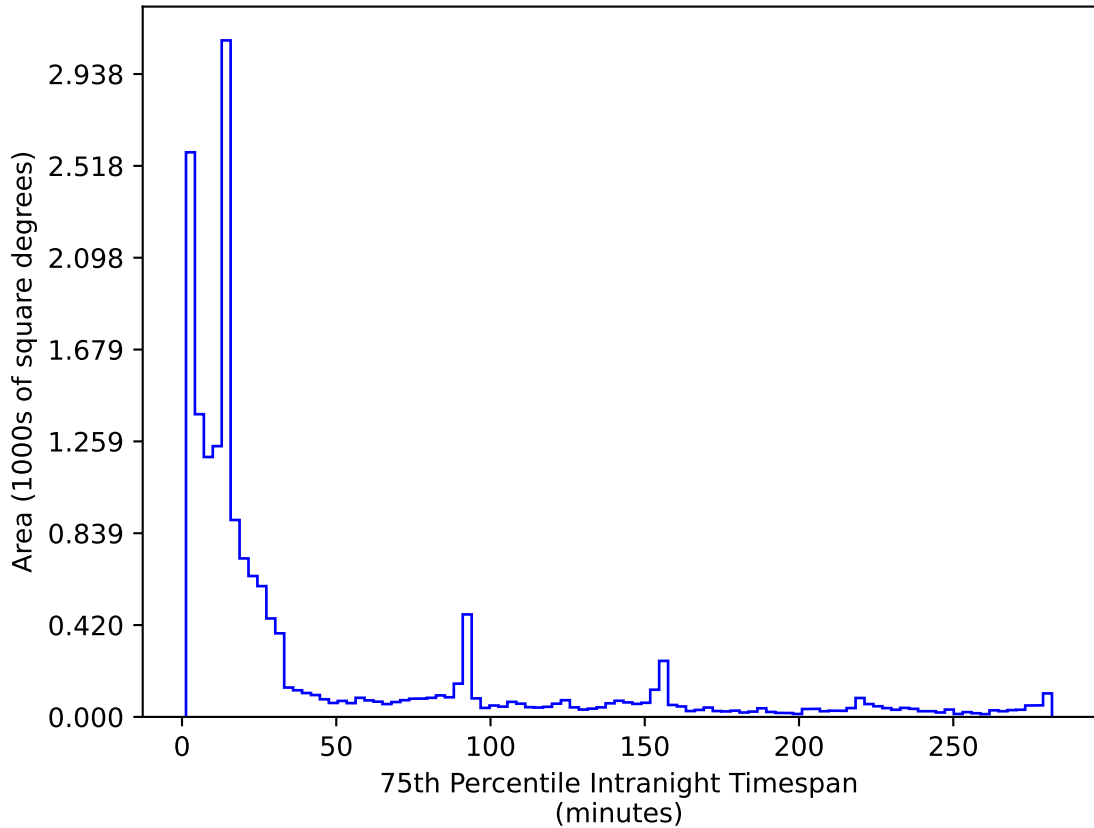
too_100_1v3.4_10yrs WFD r band: 75th Percentile Intranight Timespan
