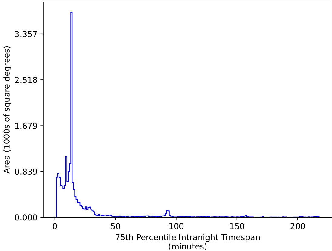
too_100_1v3.4_10yrs WFD i band: 75th Percentile Intranight Timespan
