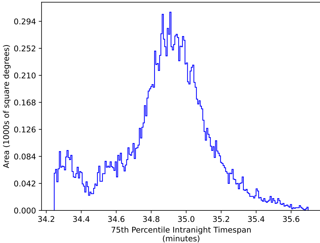
too_100_1v3.4_10yrs WFD all bands: 75th Percentile Intranight Timespan
