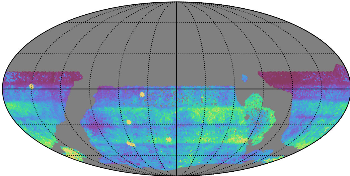
too_100_1v3.4_10yrs WFD: 75th Percentile Intranight Timespan
