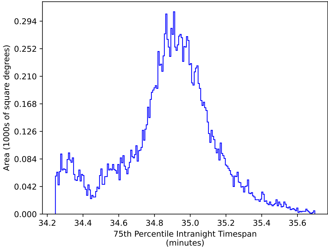
too_100_1v3.4_10yrs WFD: 75th Percentile Intranight Timespan
