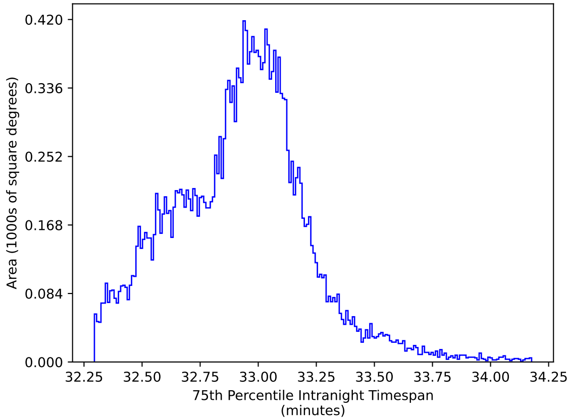
too_100_1v3.4_10yrs All sky y band: 75th Percentile Intranight Timespan
