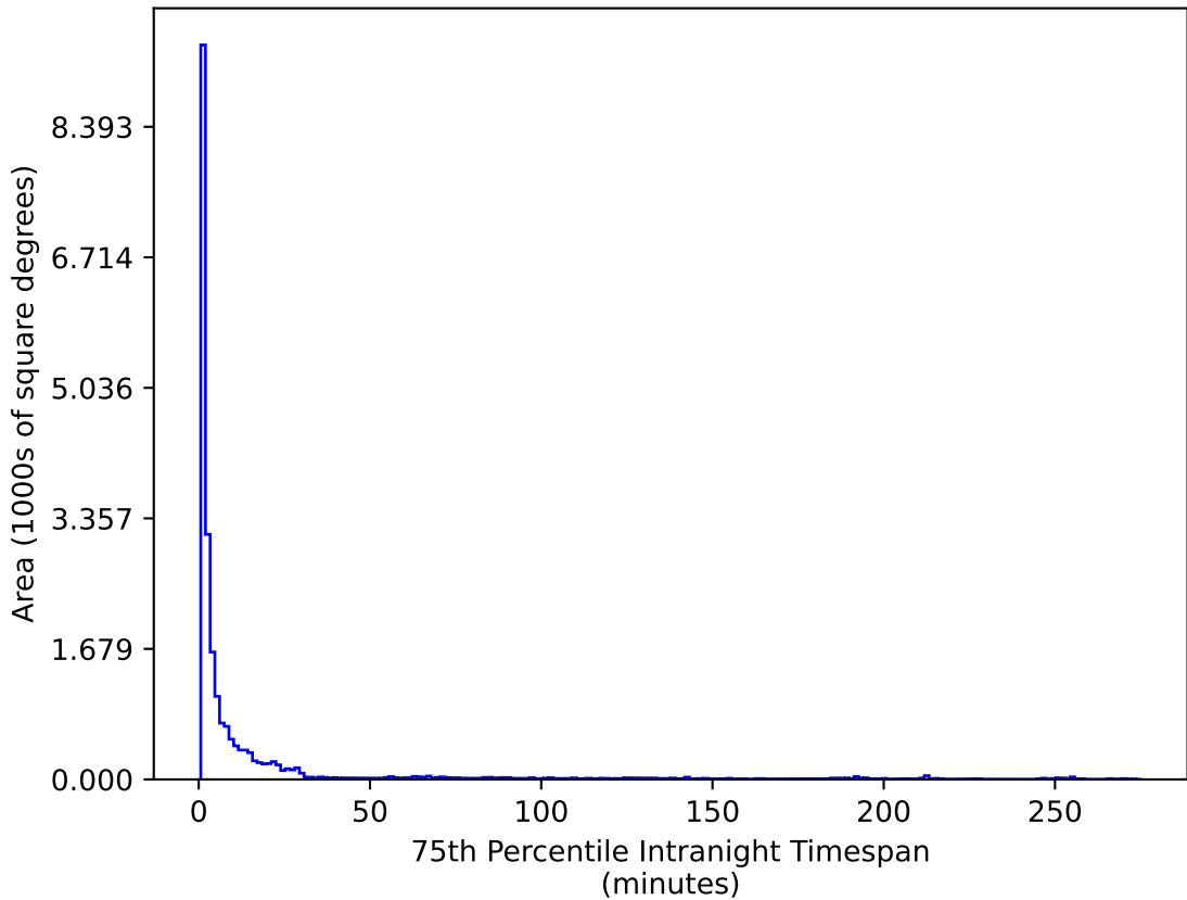
too_100_1v3.4_10yrs All sky u band: 75th Percentile Intranight Timespan
