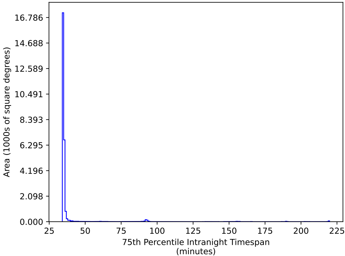
too_100_1v3.4_10yrs All sky ri bands: 75th Percentile Intranight Timespan
