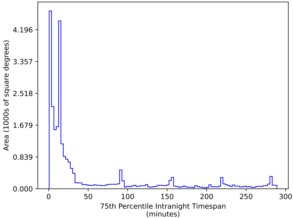
too_100_1v3.4_10yrs All sky r band: 75th Percentile Intranight Timespan
