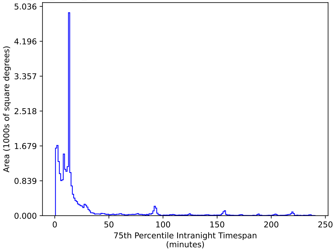
too_100_1v3.4_10yrs All sky i band: 75th Percentile Intranight Timespan
