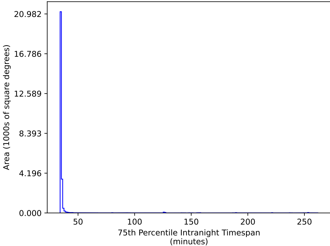
too_100_1v3.4_10yrs All sky gr bands: 75th Percentile Intranight Timespan
