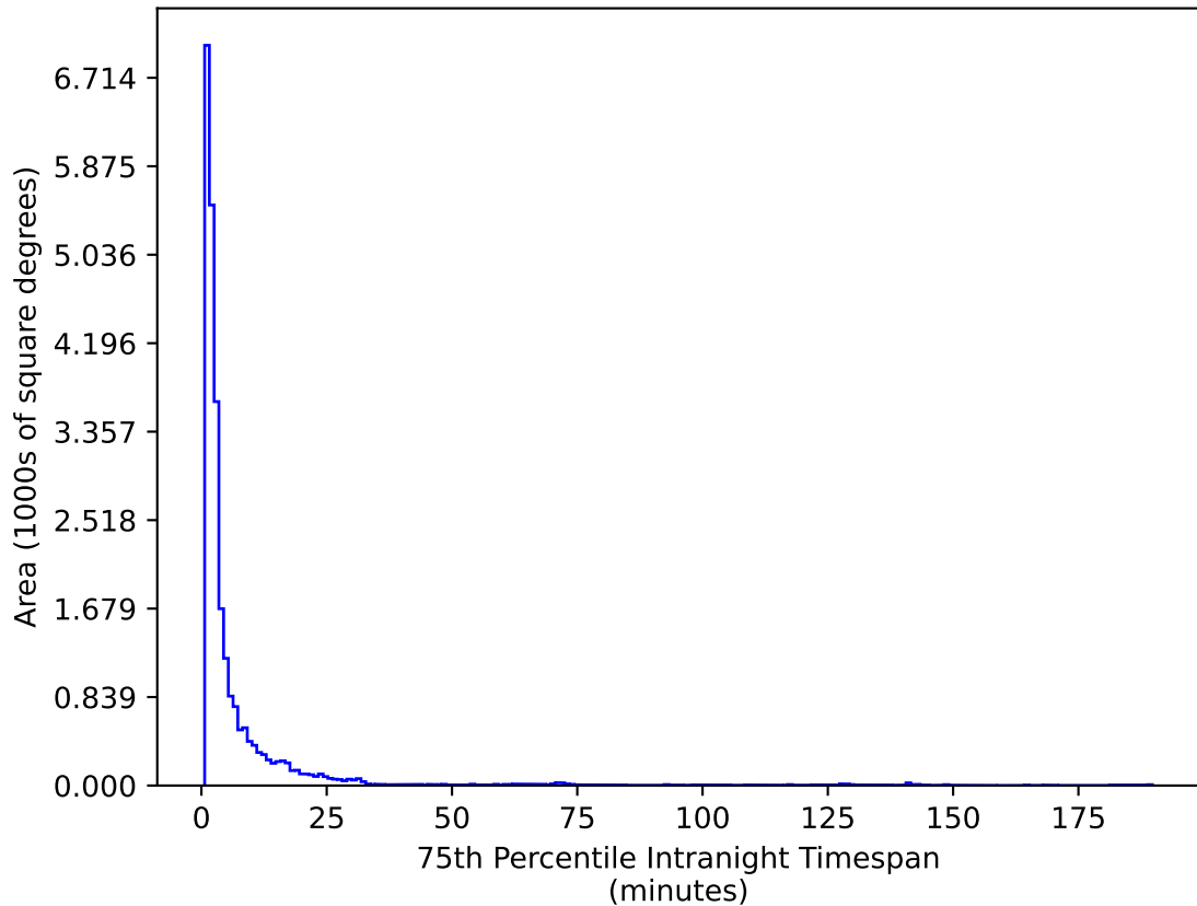
too_100_1v3.4_10yrs All sky g band: 75th Percentile Intranight Timespan
