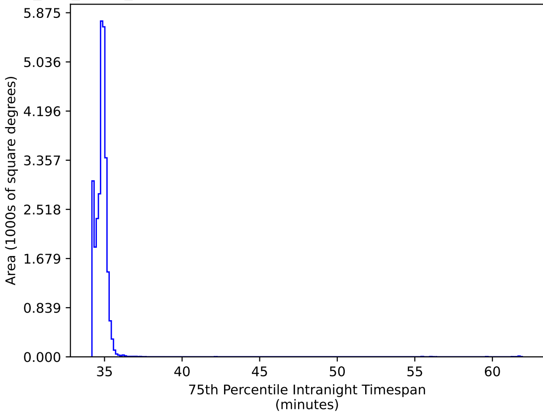
too_100_1v3.4_10yrs All sky all bands: 75th Percentile Intranight Timespan
