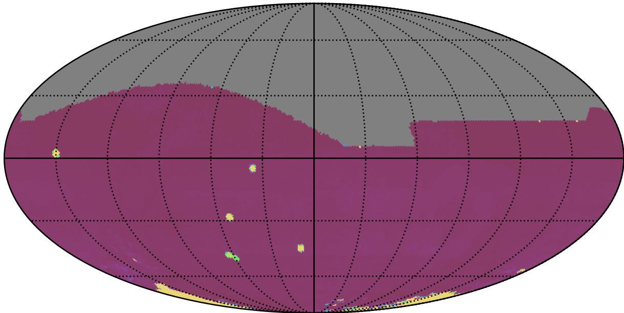
too_100_1v3.4_10yrs All sky: 75th Percentile Intranight Timespan
