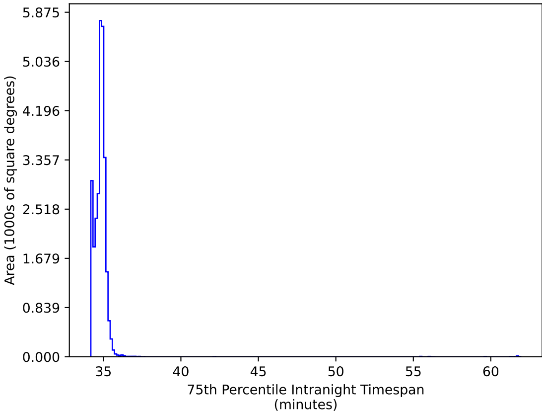
too_100_1v3.4_10yrs All sky: 75th Percentile Intranight Timespan
