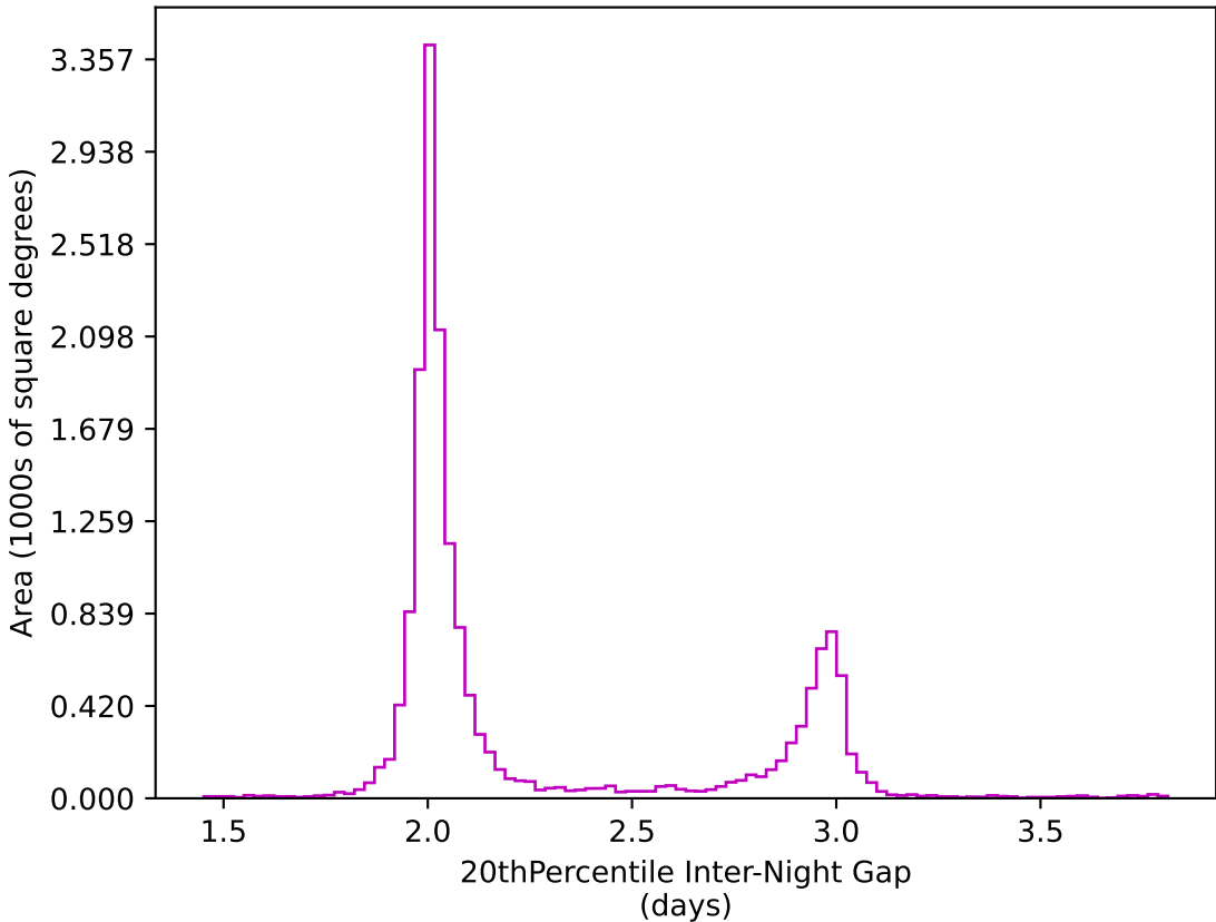
too_100_1v3.4_10yrs WFD z band: 20thPercentile Inter-Night Gap
