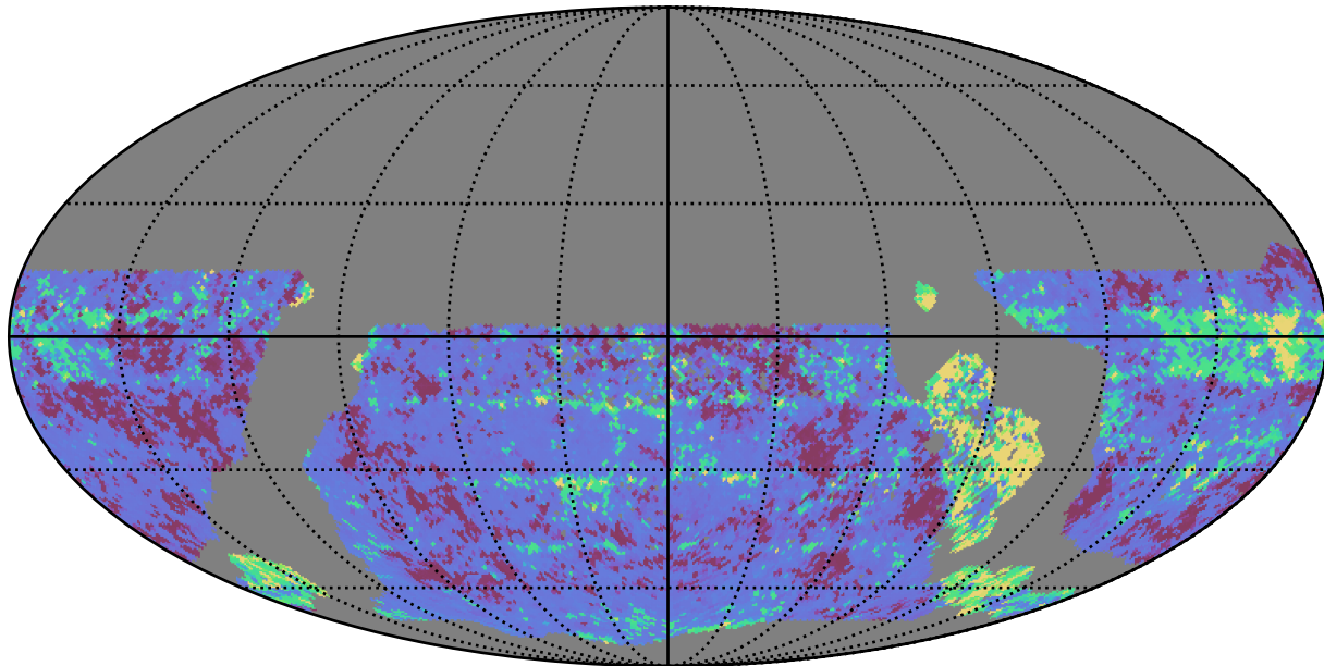
too_100_1v3.4_10yrs WFD y band: 20thPercentile Inter-Night Gap
