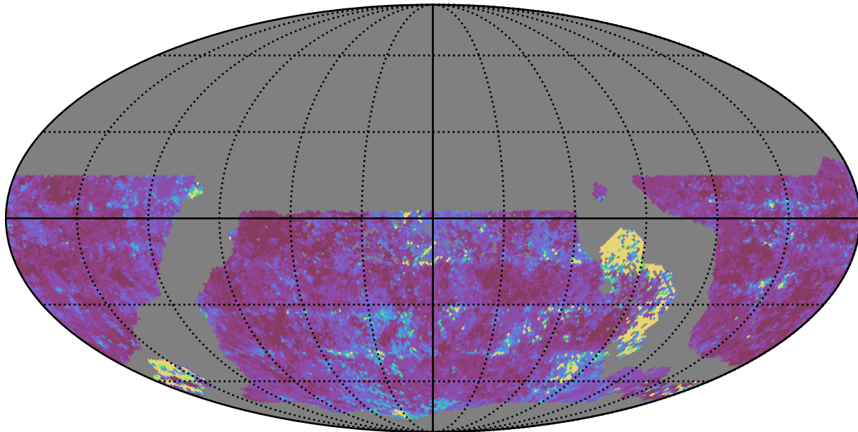
too_100_1v3.4_10yrs WFD u band: 20thPercentile Inter-Night Gap
