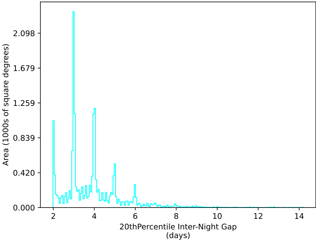
too_100_1v3.4_10yrs WFD u band: 20thPercentile Inter-Night Gap
