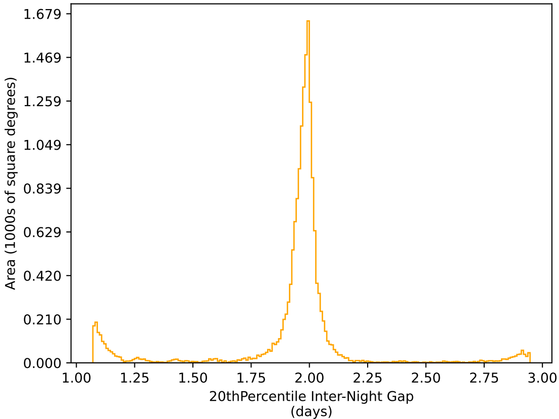
too_100_1v3.4_10yrs WFD r band: 20thPercentile Inter-Night Gap
