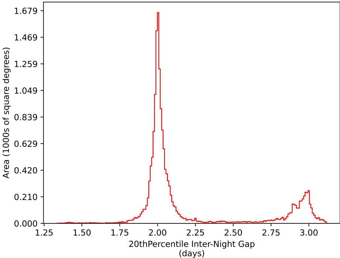
too_100_1v3.4_10yrs WFD i band: 20thPercentile Inter-Night Gap
