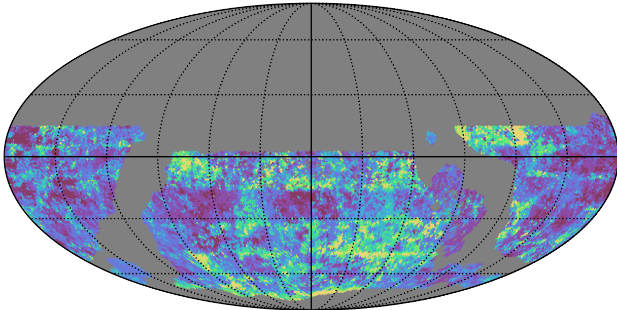
too_100_1v3.4_10yrs WFD g band: 20thPercentile Inter-Night Gap
