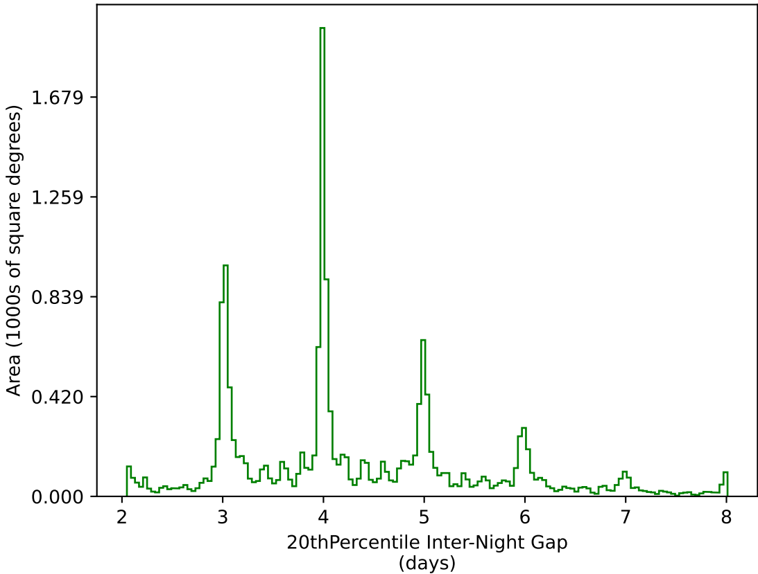
too_100_1v3.4_10yrs WFD g band: 20thPercentile Inter-Night Gap
