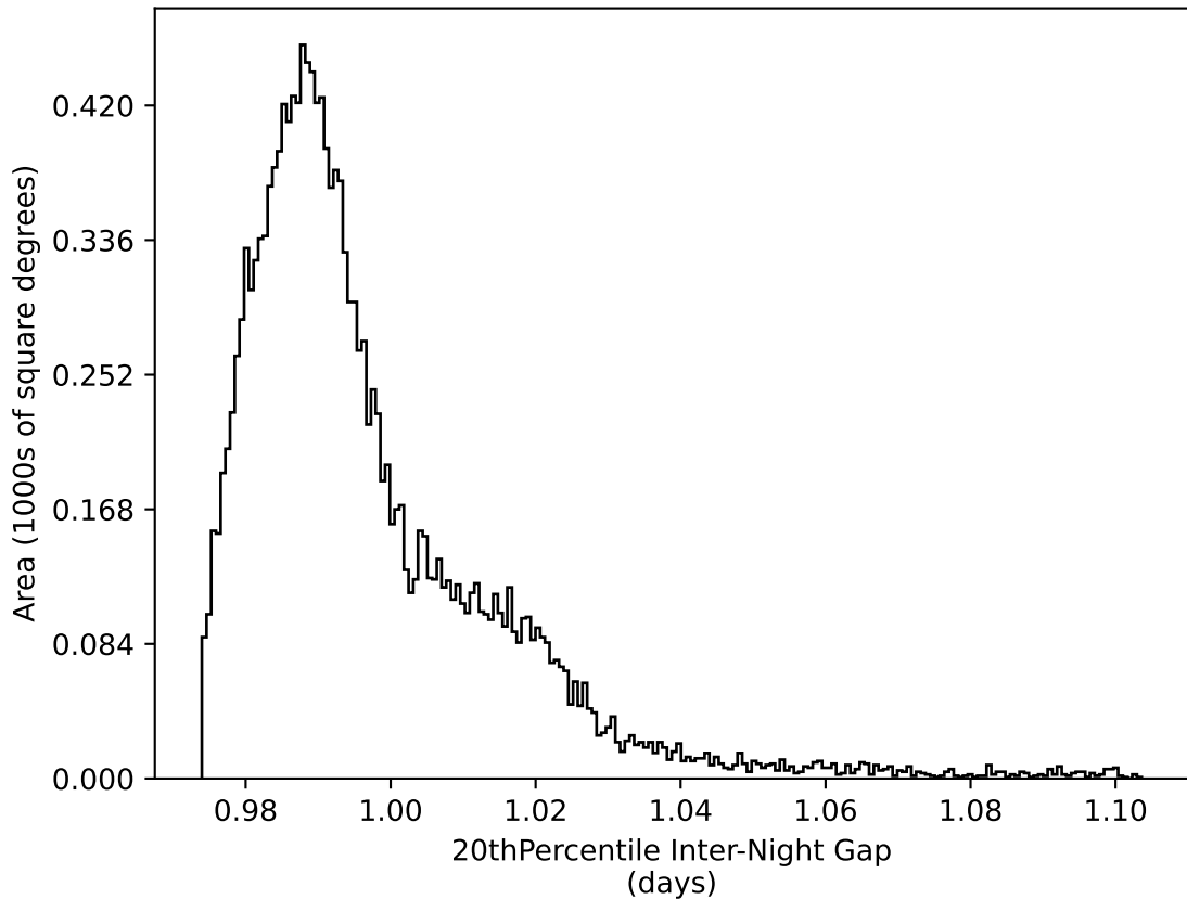
too_100_1v3.4_10yrs WFD all bands: 20thPercentile Inter-Night Gap
