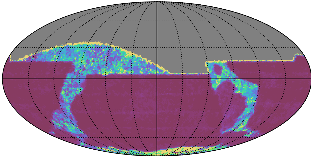
too_100_1v3.4_10yrs All sky z band: 20thPercentile Inter-Night Gap
