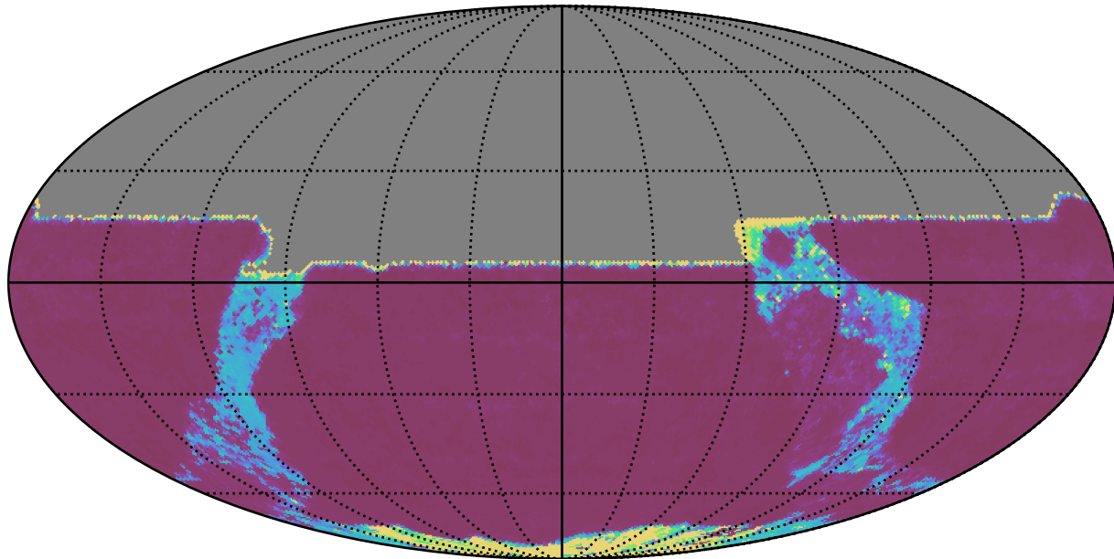
too_100_1v3.4_10yrs All sky y band: 20thPercentile Inter-Night Gap
