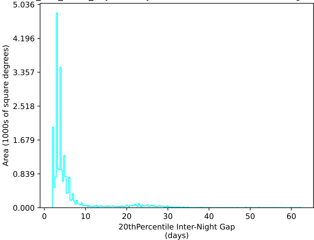
too_100_1v3.4_10yrs All sky u band: 20thPercentile Inter-Night Gap
