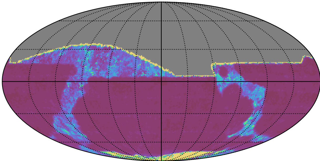
too_100_1v3.4_10yrs All sky r band: 20thPercentile Inter-Night Gap
