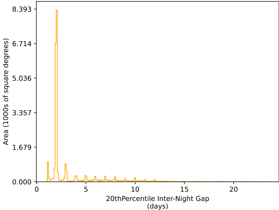
too_100_1v3.4_10yrs All sky r band: 20thPercentile Inter-Night Gap
