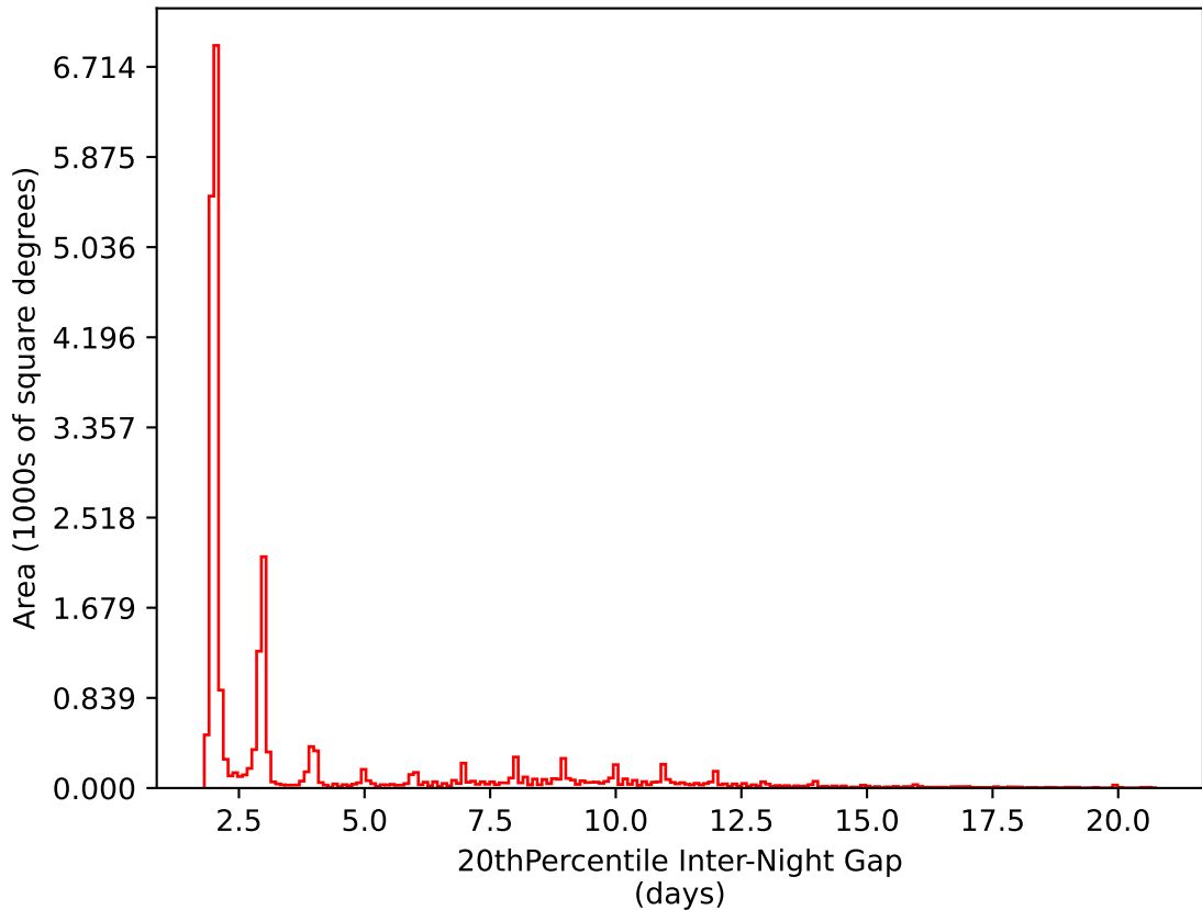
too_100_1v3.4_10yrs All sky i band: 20thPercentile Inter-Night Gap
