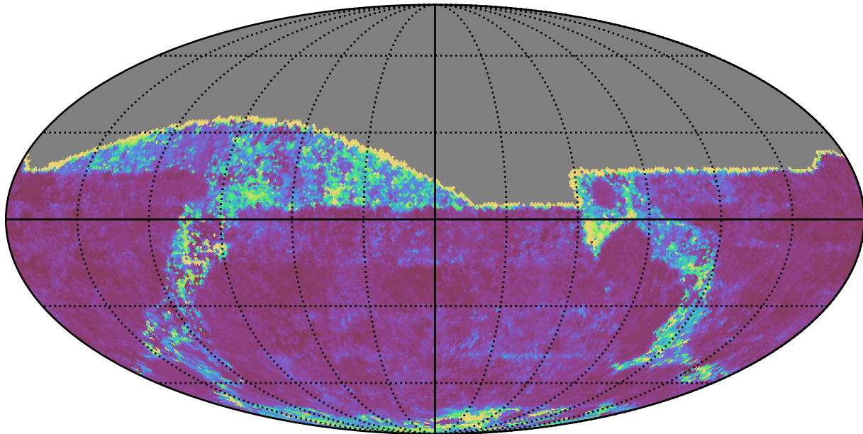
too_100_1v3.4_10yrs All sky g band: 20thPercentile Inter-Night Gap
