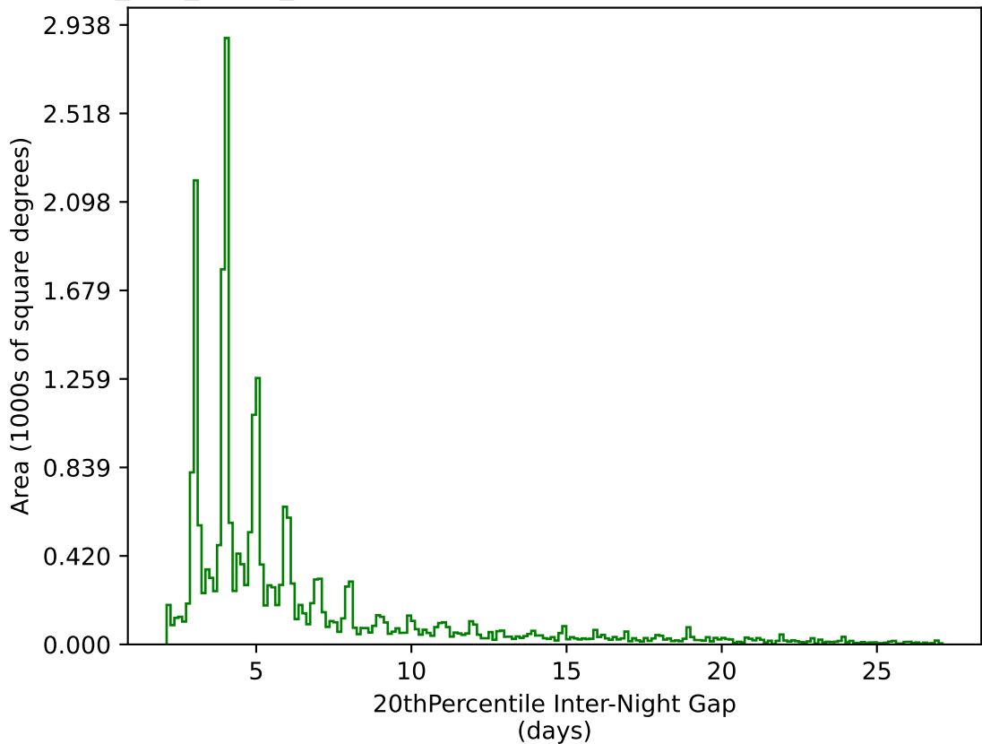
too_100_1v3.4_10yrs All sky g band: 20thPercentile Inter-Night Gap
