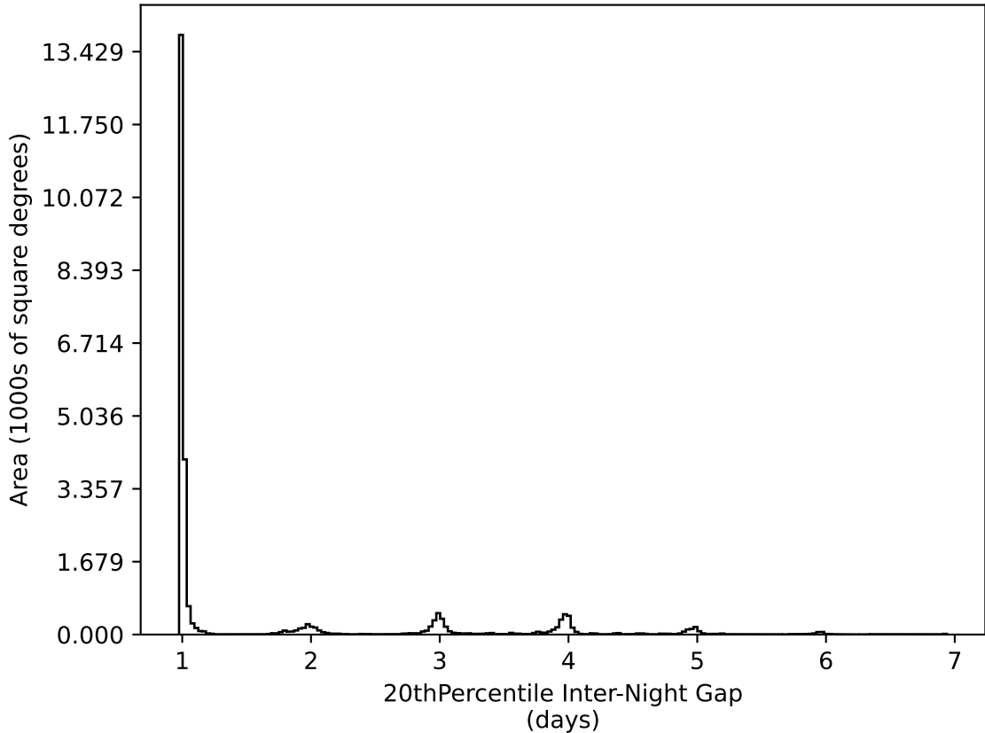
too_100_1v3.4_10yrs All sky all bands: 20thPercentile Inter-Night Gap
