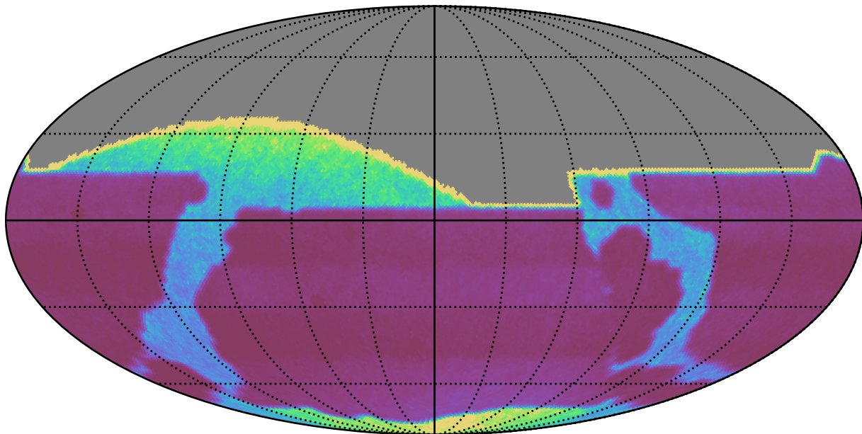
too_100_1v3.4_10yrs : properMotion
