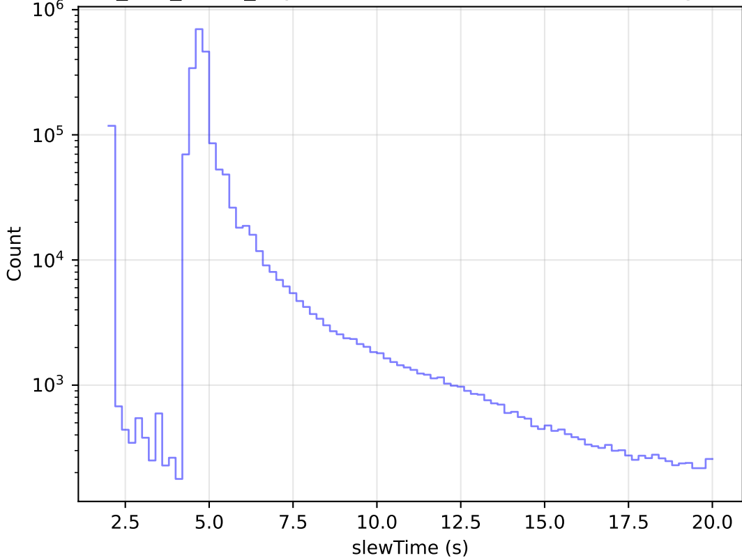
too_100_1v3.4_10yrs All visits: Zoom Slew Time Histogram
