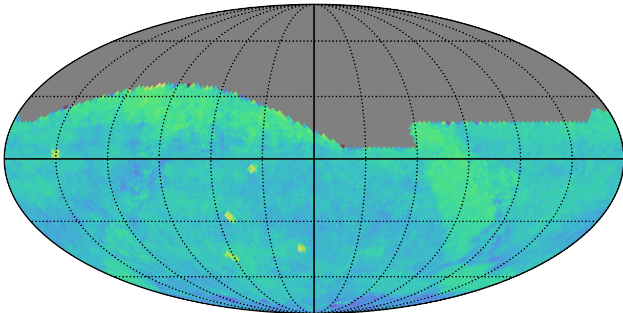
too_100_1v3.4_10yrs (g or r or i): PairFraction
