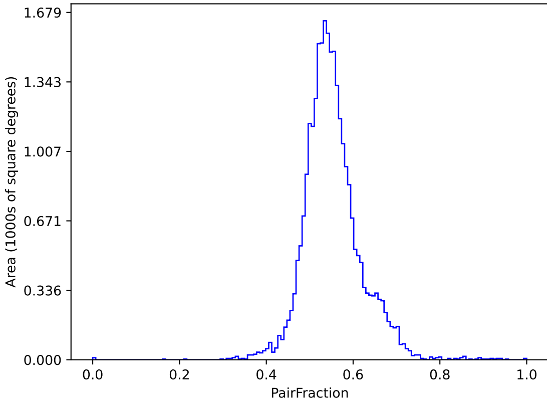
too_100_1v3.4_10yrs (g or r or i): PairFraction
