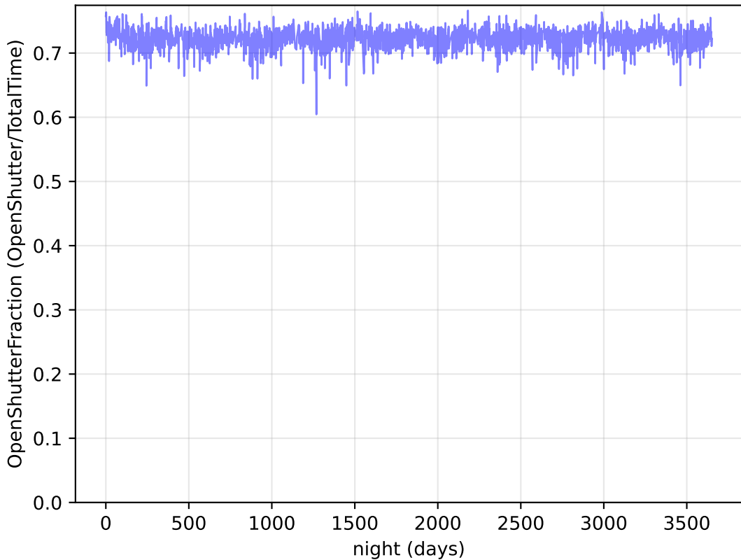
too_100_1v3.4_10yrs : OpenShutterFraction
