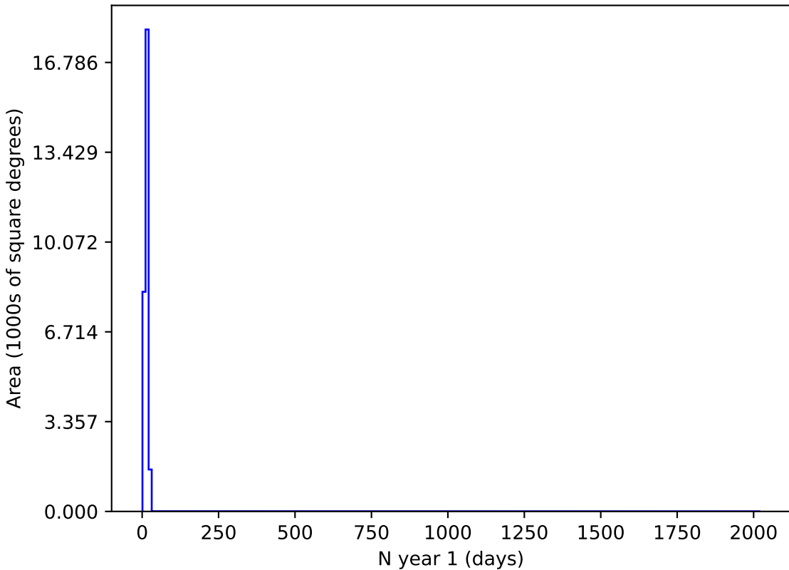
too_100_1v3.4_10yrs z and night < 365: N year 1
