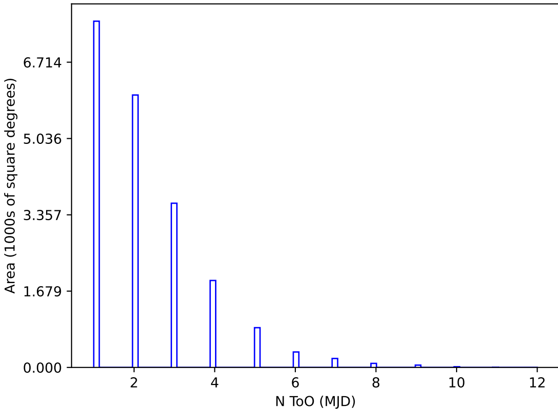
too_100_1v3.4_10yrs z and note like ToO%: N ToO
